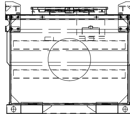
VIEW A-A (SIDE)
