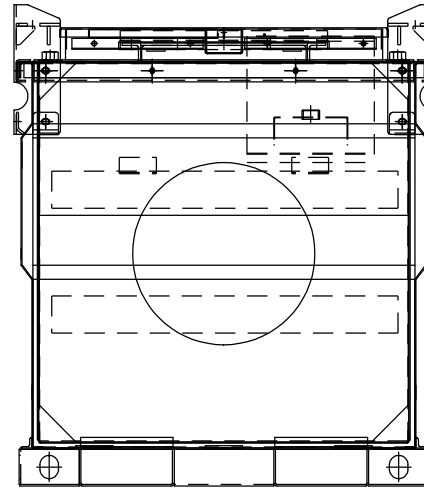
VIEW A-A (SIDE)
